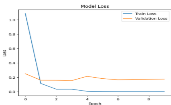
Fig. 20. Loss graph of VGC 16 classifier
