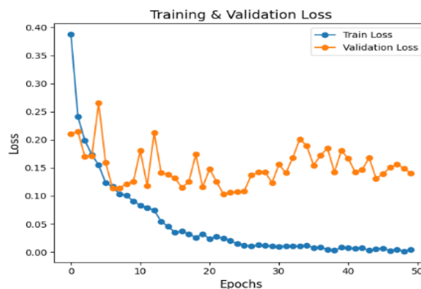
Fig. 22. Loss graph of CNN classifier
