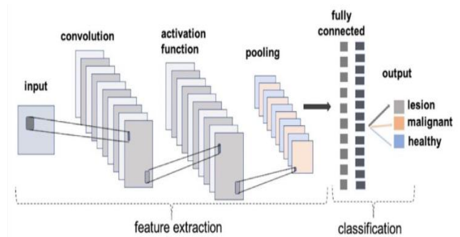
Fig. 12. Architecture of CNN model
