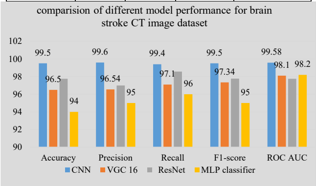
Fig. 23. Comparison of model performance metrics
